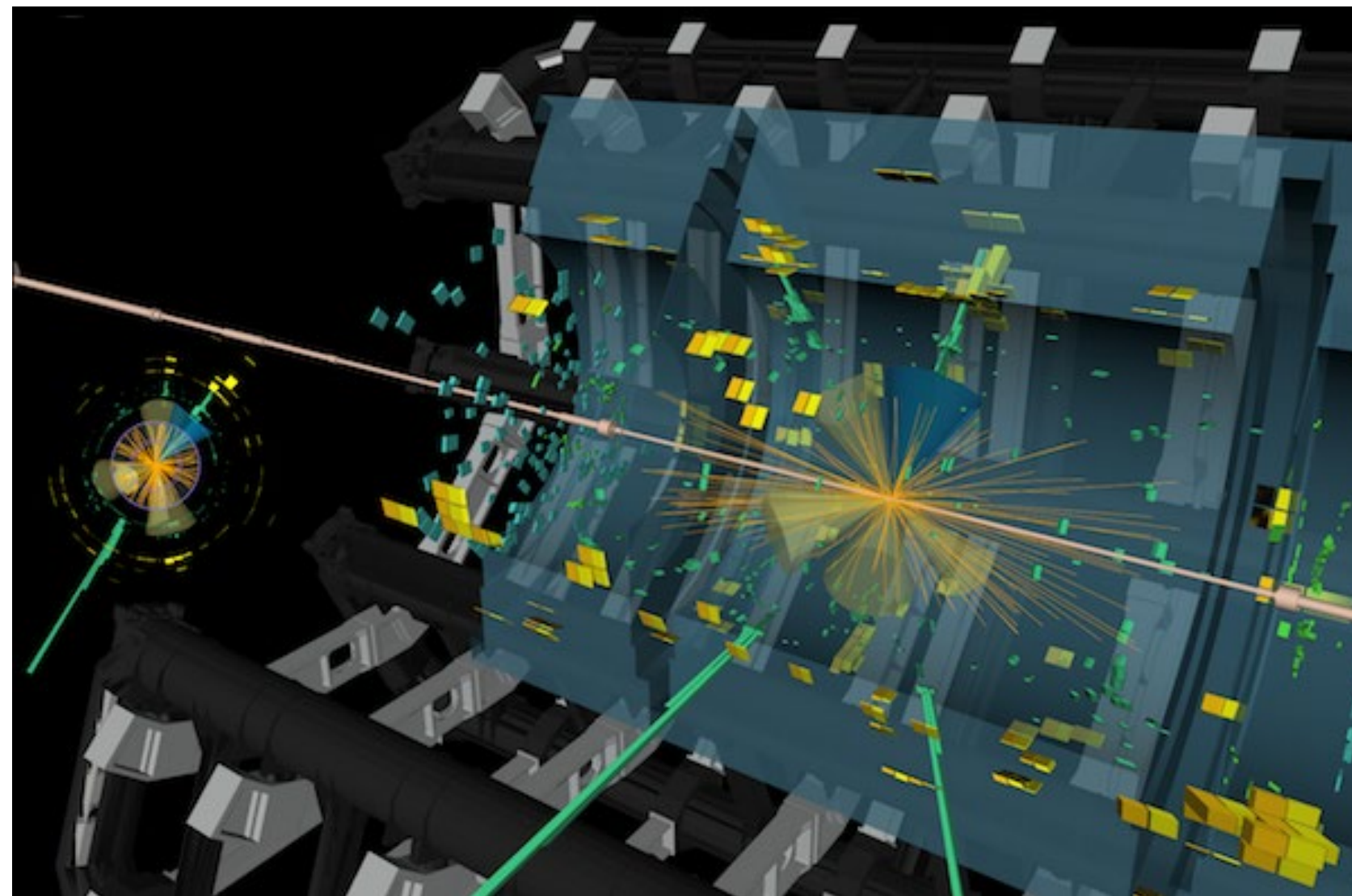
Visualization of an event from the t\bar{t} H(\gamma\gamma) analysis. The event contains two photon candidates displayed as green towers in the electromagnetic calorimeter, and six jets (b-jet) shown as yellow (blue) cones.
